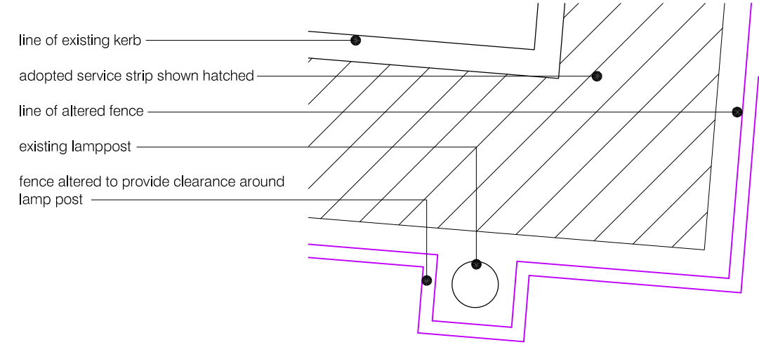
proposed plan excerpt scale 1:20
