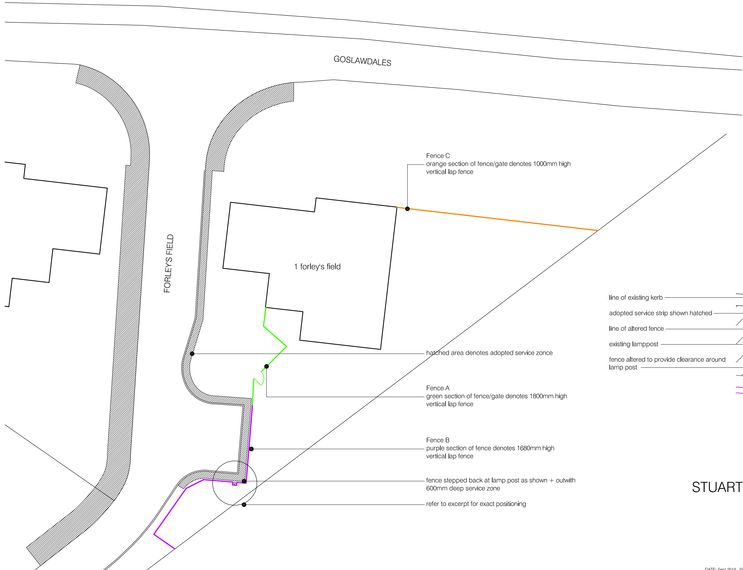
proposed part plan scale 1:200
